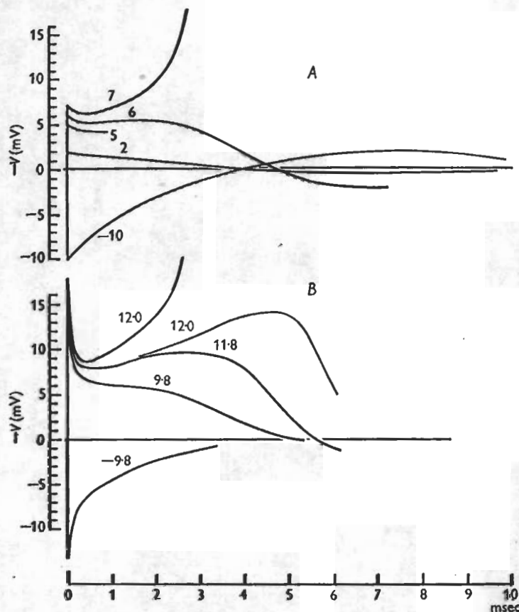
Fig. 21. A , numerical solutions of eqn. (26) for 6°C. The numbers attached to the curves give the initial depolarization in mV (also the quantity of charge applied in \mu\text{coulomb/cm}^2 ). B , response of nerve membrane at 6°C to short shocks; the numbers show the charge applied in \mu\text{coulomb/cm}^2 . The curves have been replotted from records taken at low amplification and a relatively high time-base speed.
