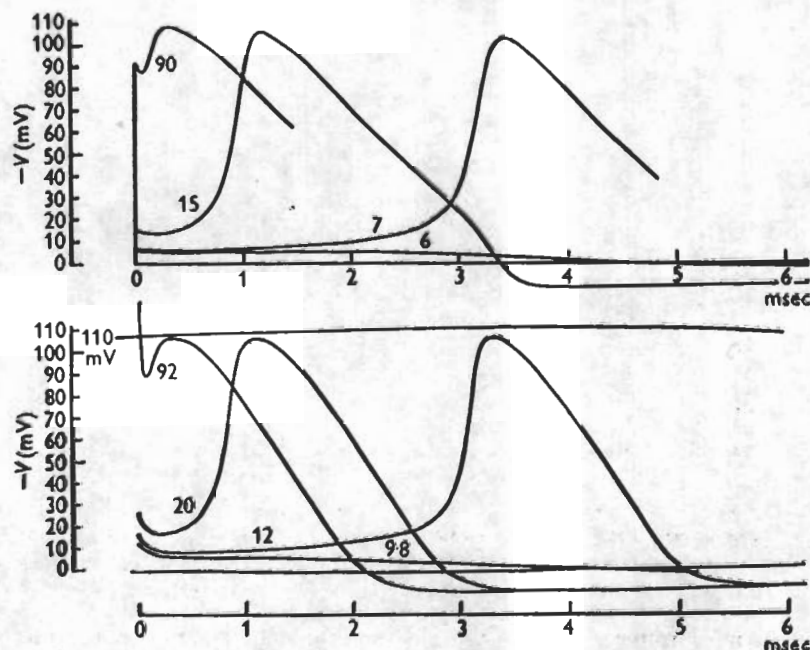
Fig. 12. Upper family: solutions of eqn. (20) for initial depolarizations of 90, 15, 7 and 6 mV (calculated for 6° C). Lower family: tracings of membrane action potentials recorded at 6° C from axon 17. The numbers attached to the curves give the shock strength in \mu\text{coulomb/cm}^2 . The vertical and horizontal scales are the same in both families (apart from the slight curvature indicated by the 110 mV calibration line). In this and all subsequent figures depolarizations (or negative displacements of V ) are plotted upwards.
