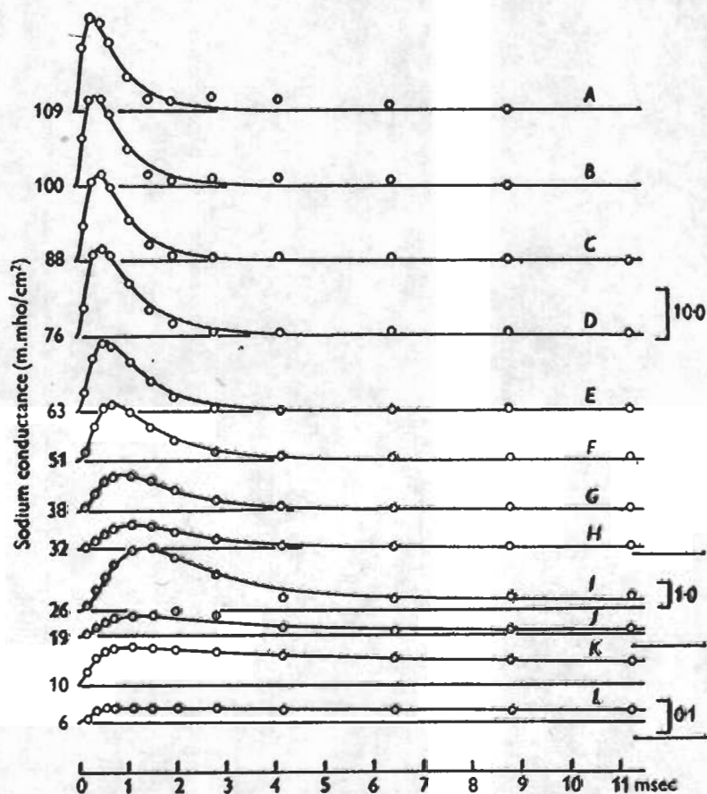
Fig. 6. Changes of sodium conductance associated with different depolarizations. The circles are experimental estimates of sodium conductances obtained on axon 17, temperature 6-7° C (cf. Fig. 3). The smooth curves are theoretical curves with parameters shown in Table 2; A to H drawn from eqn. 19, I to L from 14, 17, 18 with \bar{g}_{Na} = 70.7 m.mho/cm 2 . The ordinate scales on the right are given in m.mho/cm 2 . The numbers on the left show the depolarization in mV. The time scale applies to all curves.
